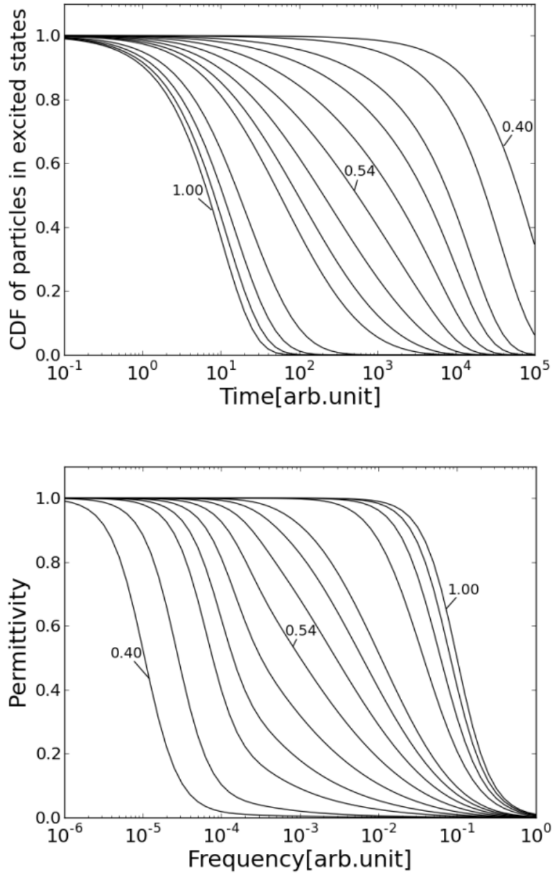
Figure 8.1 a=0.40, 0.44, 0.48, 0.50, 0.52, 0.54, 0.56, 0.58, 0.60, 0.70, 0.80, 0.90, 1.00 (only 0.40, 0.54 and 1.00 curves are indicated in figures.) and g_0=0.1, \Gamma_0=0.1, b=0.5 . Top: CDF curves. As value of a increases, the curves shift to the shorter time. Bottom: Permittivity curves. As value of a increases, the curves shift to the higher frequency.
