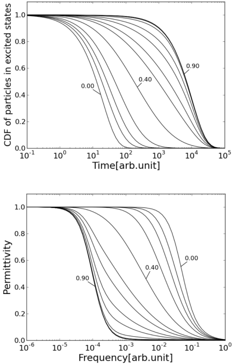
Figure 8.2 b = 0.00, 0.10, 0.20, 0.30, 0.40, 0.45, 0.47, 0.50, 0.53, 0.60, 0.70, 0.80, 0.90 (only 0.00, 0.40 and 0.90 curves are indicated in figures.) and g_0=0.1, \Gamma_0=0.1, a = 0.5 . Top: CDF curves. As value of b increases, the curves shift to the longer time. Bottom: Permittivity curves. As value of b increases, the curves shift to the lower frequency.
