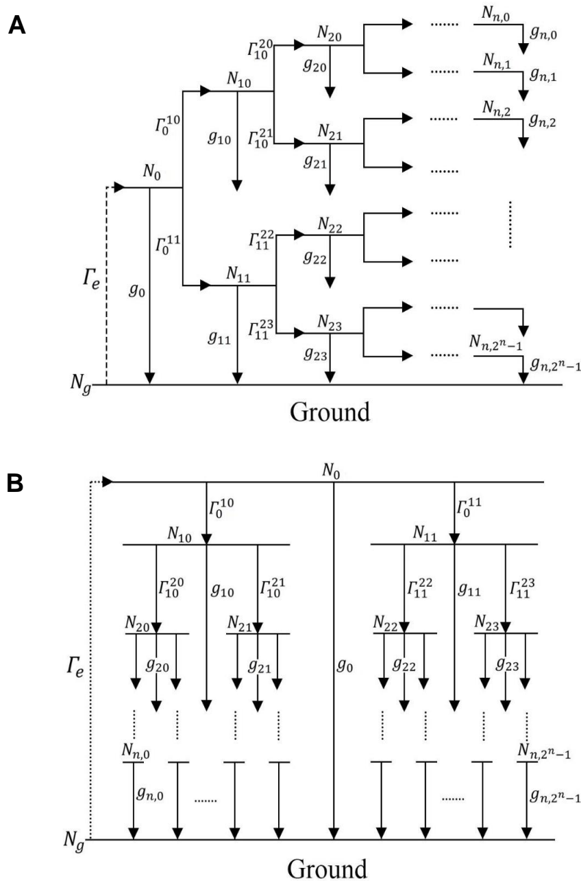
Figure 7.5 Catorian tree type fractal network from the 0-th to n -th generation. N_g, N_{\alpha\beta}, \Gamma_{\alpha\beta}, g_{\alpha\beta} ( \alpha = 0, 1, 2, \dots, n , \beta = 0, 1, \dots, 2^\alpha - 1 ) are the number of particles in ground state, the number of particles in one of branches of the generation, the transfer rate from a branch to another, the de-excitation rate from a branch to the ground state. Superscripts of the transfer rate, \Gamma , denote the branch that particles flow into. \Gamma_e is the excitation rate from the ground state to the 0th generation. Panel A shows an example of a Cantorian network evenly branching such as blood vessels in the lungs placed between a pair of electrodes [3]. Panel B shows another example in which particles such as electrons in excited states flow down hierarchically through a system of energetic levels (many of which are degenerate) from one with higher energy to another one with lower energy and then further down to the ground state.
