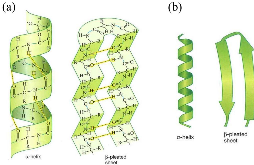
Figure 1.4 Secondary structures of proteins. \alpha -helix and \beta -pleated sheet are shown in (a) explicit representation of chemical structures with hydrogen bonds (yellow dashed-line), and (b) schematic representation, the so-called ribbon or cartoon diagram, commonly used to express secondary structures, where arrowheads are at the carboxyl end of the arrows in \beta -sheet. FREEMAN, SCOTT, BIOLOGICAL SCIENCE, 2 nd Edition, © 2005 [6]. Reprinted and Electronically reproduced by permission of Pearson Education, Inc., Upper Saddle River, NJ.
